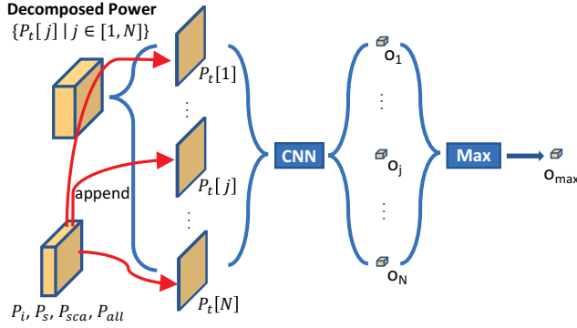
Fig. 3: PowerNet structure.
