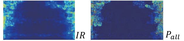
Fig. 12: Power and IR drop of vector-based estimation.
