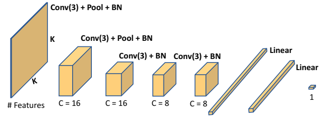
Fig. 4: CNN structure.
