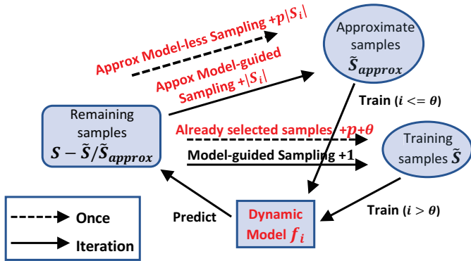
Fig. 3: FIST framework.
