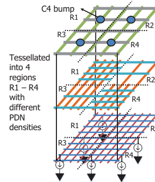
Figure 1: A template-based PDN with piecewise uniform pitches. Specifically, this work tessellates the entire chip into rectangular regions (Fig. 1), each of which uses one of the templates; different regions may use different templates. This resembles the idea of locally regular, globally irregular grids in [10] for two top-level metal layers, but we (i) use a limited set of templates, and (ii) apply this approach across the entire interconnect stack. The PDN design problem then reduces to mapping templates to regions of the chip.
