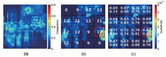
Figure 9: CNN-based demonstration of the inference scheme at the placement stage of Core1 [11]: (a) input signal congestion map, (b) current distribution and the synthesized template-based PDN, (c) average congestion (signal + PDN) in every region after classification of different templates (top number); average congestion (signal + PDN) in every region after using a uniform PDN across the entire die (bottom number).
