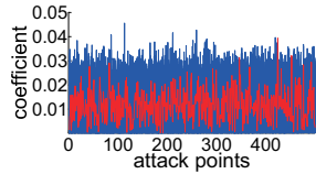
(c) CEMA results of the AES_CEP.
