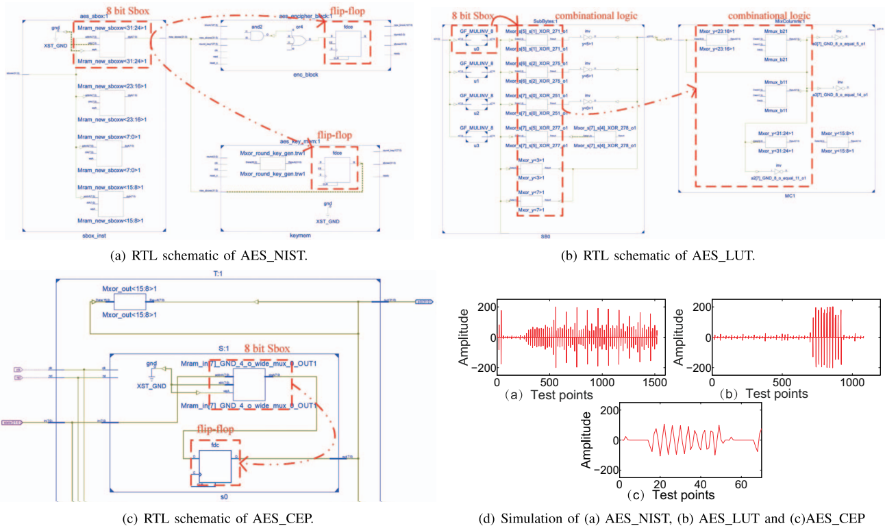
Fig. 2. RTL schematics of AES_NIST, AES_LUT, AES_CEP, and their respective simulation traces.
