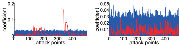
(a) CEMA results of the AES_NIST. (b) CEMA results of the AES_LUT.
